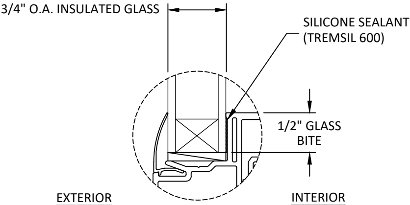
GLAZING DETAIL 1
