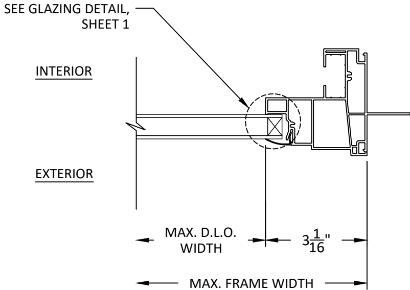
E 4 HORIZONTAL SECTION FIXED JAMB
