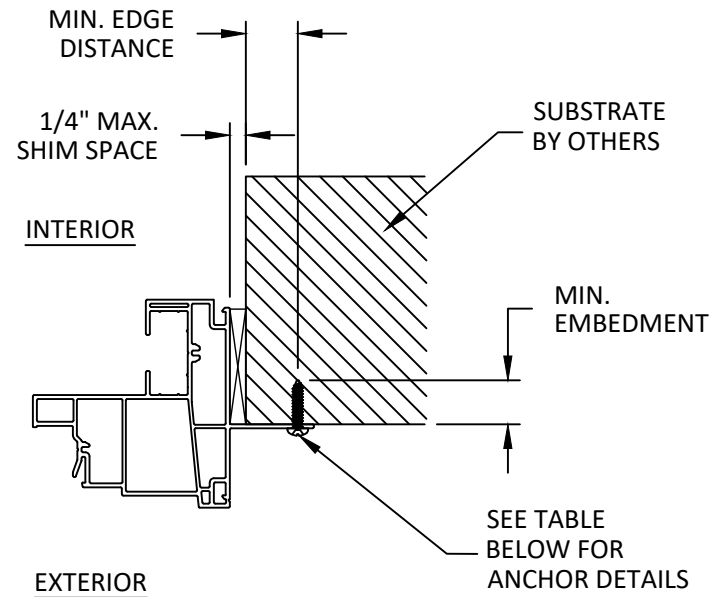
C 5 HORIZONTAL SECTION JAMB INSTALLATION
