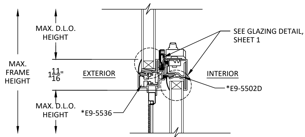
B 3 VERTICAL SECTION INTERLOCK RAIL
