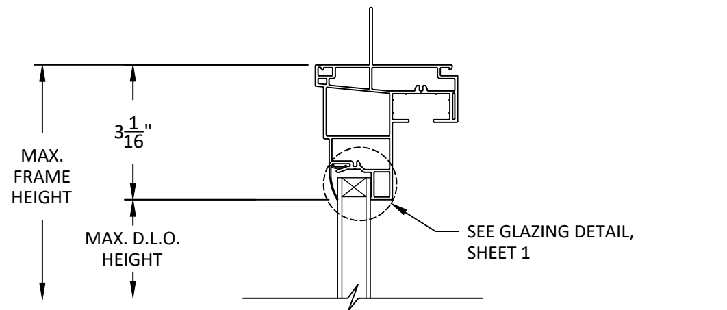
A 3 VERTICAL SECTION HEAD
