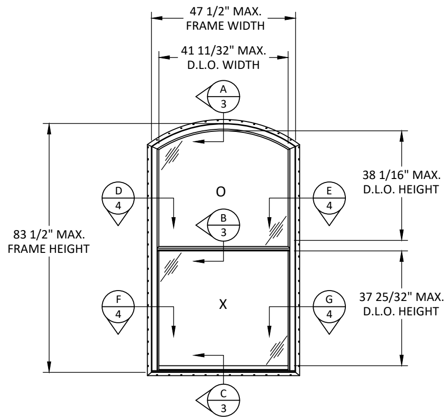
ELEVATION TYPICAL
