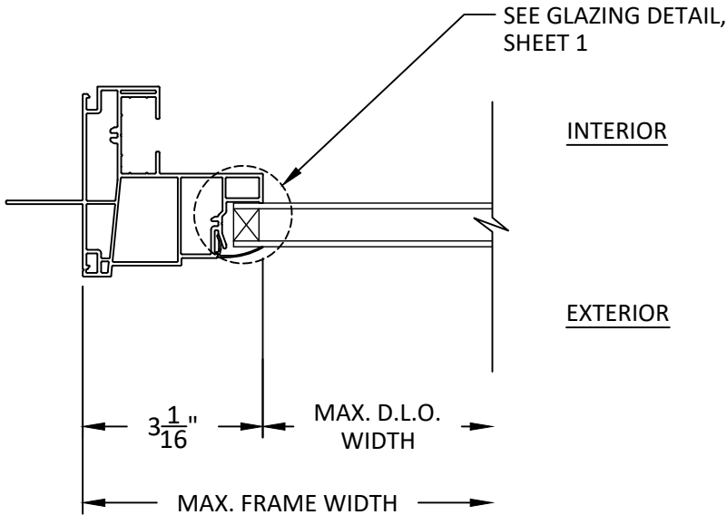
D 4 HORIZONTAL SECTION FIXED JAMB
