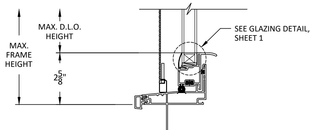
C 3 VERTICAL SECTION SILL
