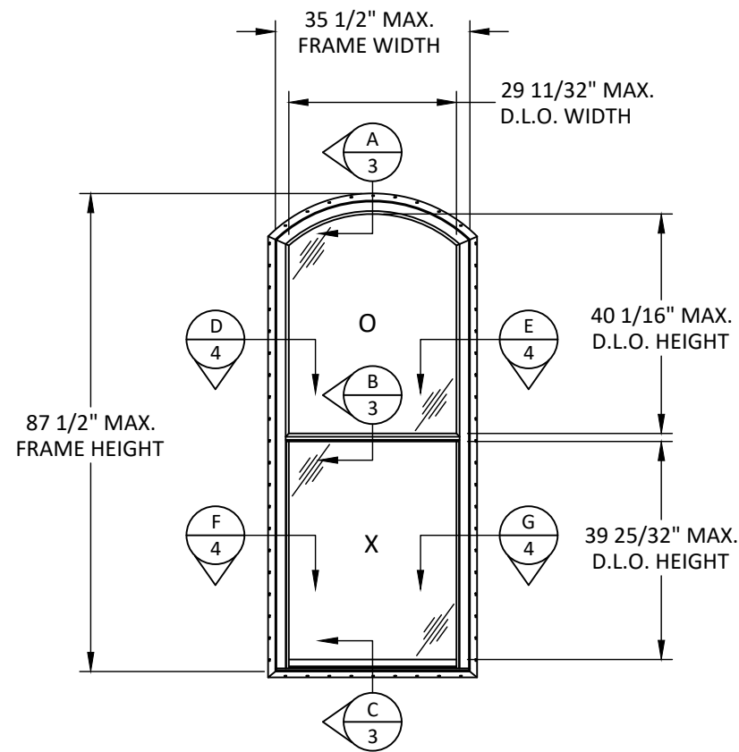
ELEVATION TYPICAL
